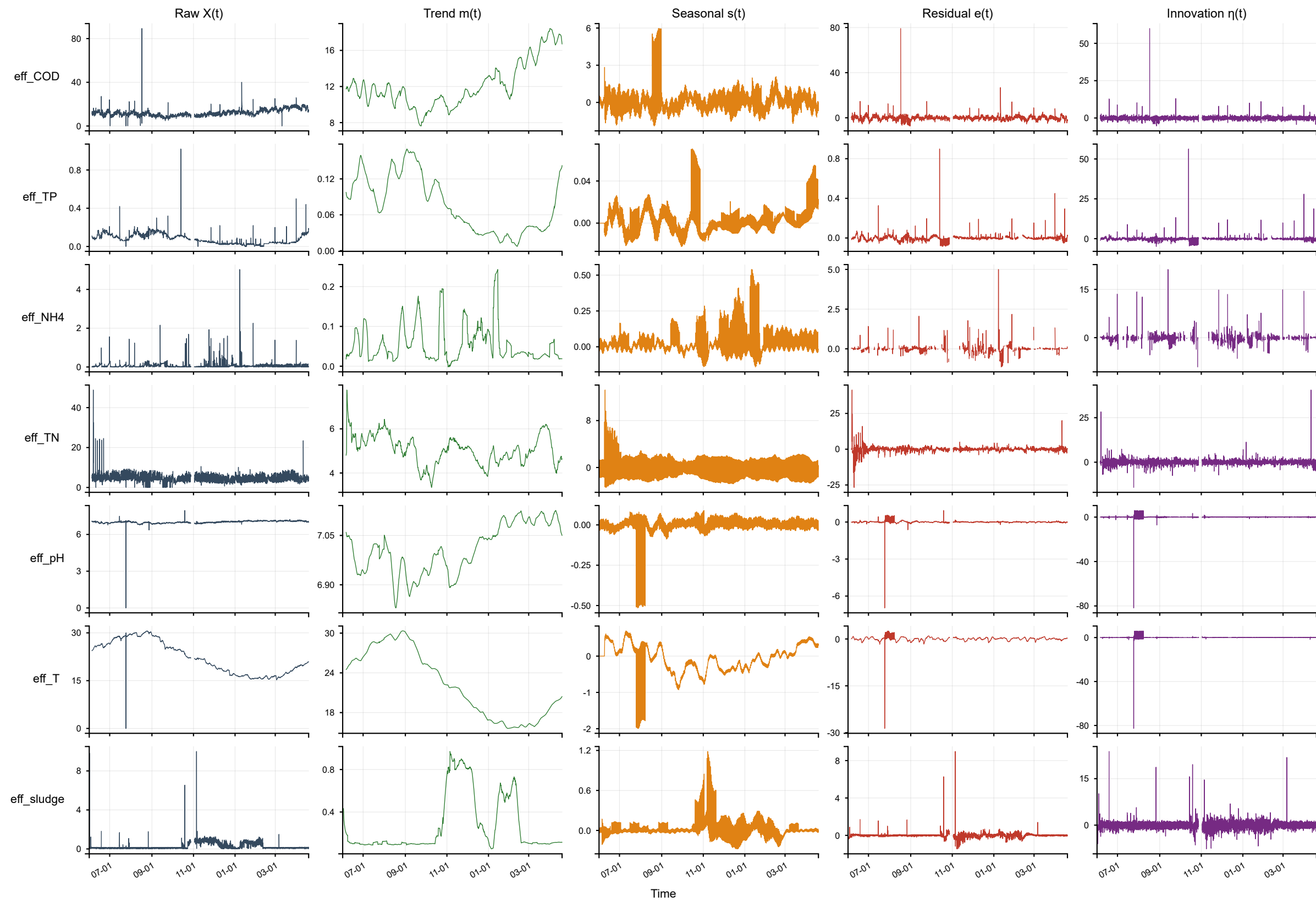
Effluent water-quality variables — trend/seasonal/residual/innovation grid [2025-06-01~2026-04-19]
